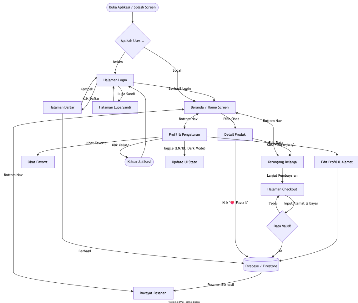
Figure 4.2 – System Flowchart
